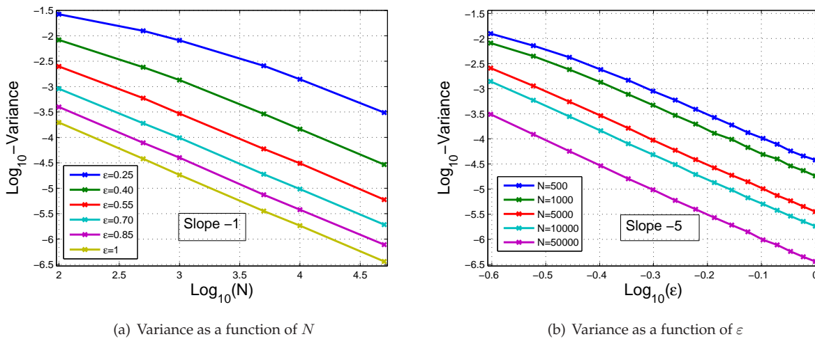
Figure 1: Variance error as a function of the number of particles, N , and the mollifier window width, \varepsilon , for dimension d = 5 at the final time step T = 1 .
